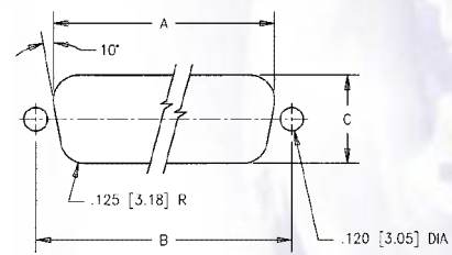
OPTIONAL CUT-OUT (FOR REAR MOUNTING)
