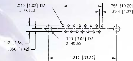
Standard PCB layout
