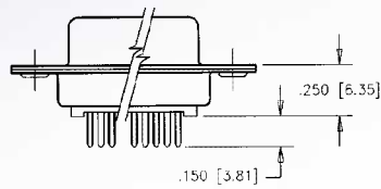
Termination Type E
