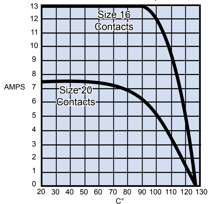
Rated Current Versus Temperature
