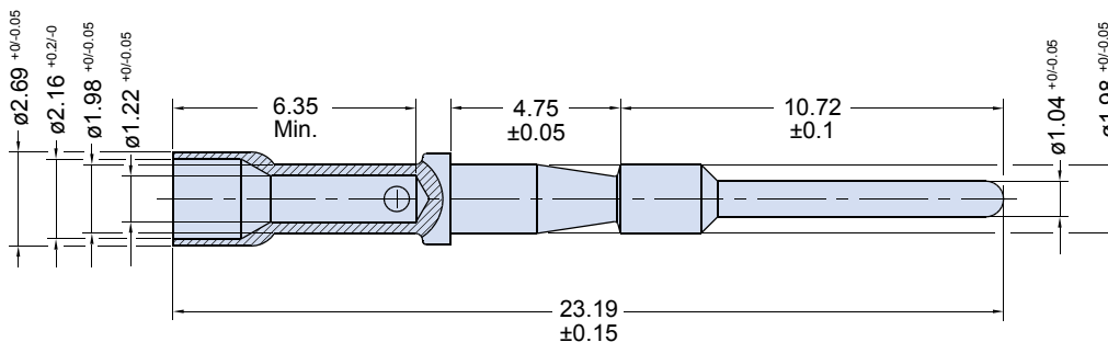
Size 20 Pin Contact 10-314980-20P
