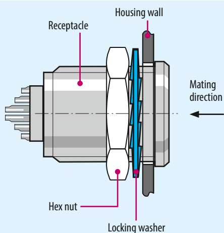
Mounting example
