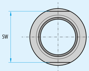
Back nut
