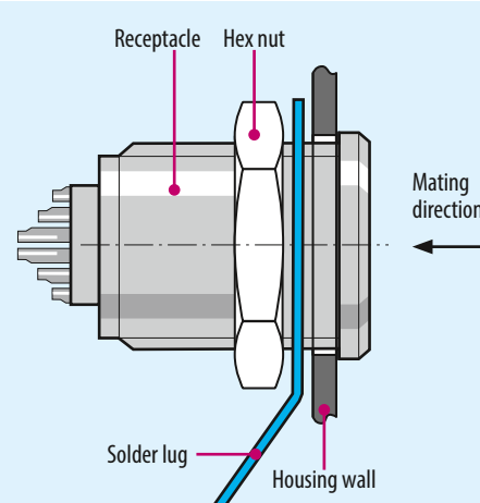
Mounting example
