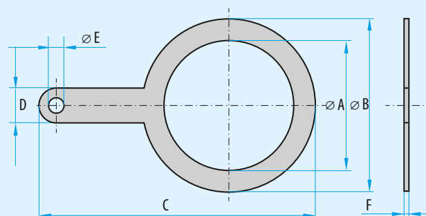
Solder lugs
