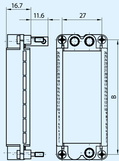
Socket frame
