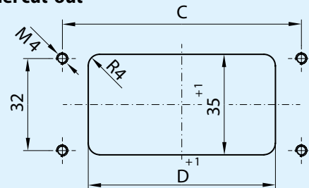
Panel cut-out
