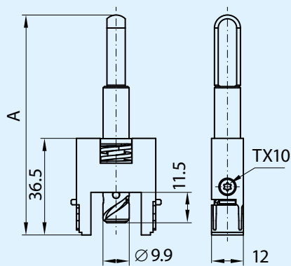
Spindle 11.5 mm
