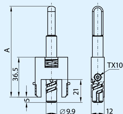
Spindle 21 mm
