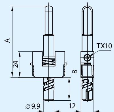
Spindle 21 mm
