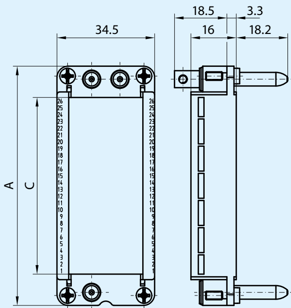
Pin frame
