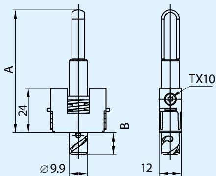
Spindle 12 mm
