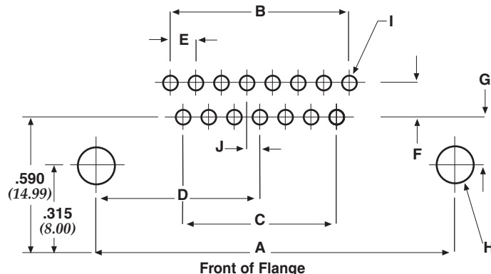
Printed Circuit Right Angle Mount (standard density)
