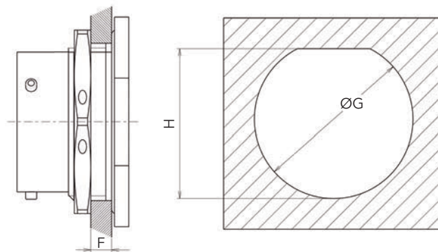
Panel cut-out
