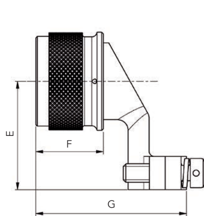
Elbow cable clamp (type 51-1)
