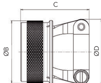
Straight cable clamp (types 02 & 52-1)
