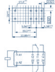
Pin layout | circuit diagram
