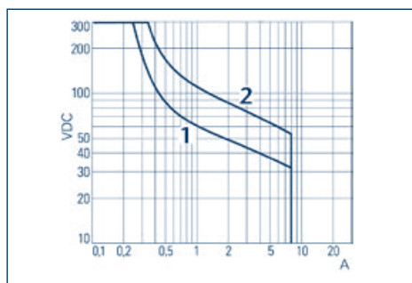
Switching capacity under DC load Resistive load
