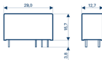
Relay - complete view
